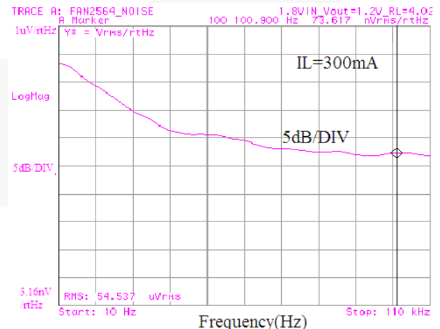
Figure 22. Noise Density
