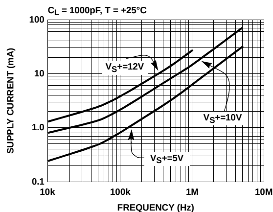
FIGURE 10. SUPPLY CURRENT vs FREQUENCY
