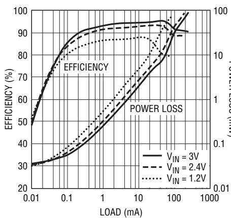
LTC3525-3.3 Efficiency and Power Loss vs Load
