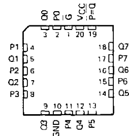
SN54LS688 . . . FK PACKAGE (TOP VIEW)
