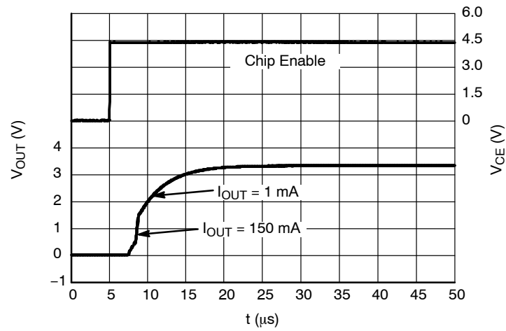
Figure 50. Start-up, 3.3 V Version, V_{IN} = 4.3\text{ V}
