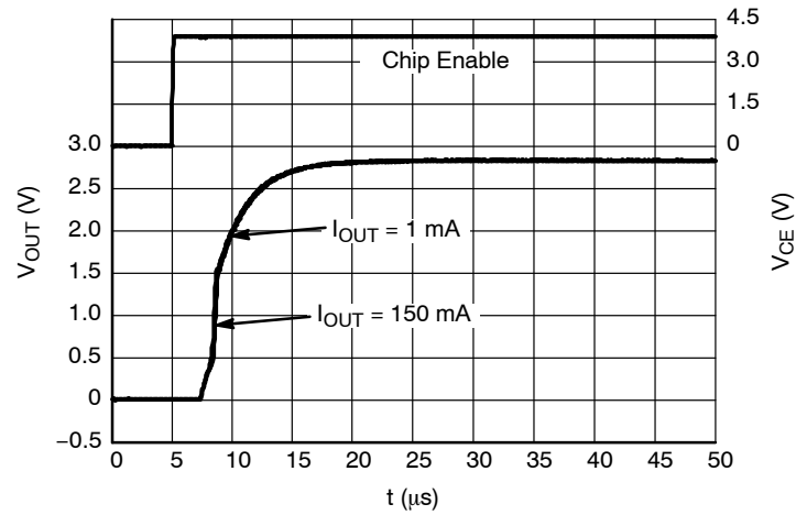
Figure 49. Start-up, 2.8 V Version, V_{IN} = 3.8\text{ V}
