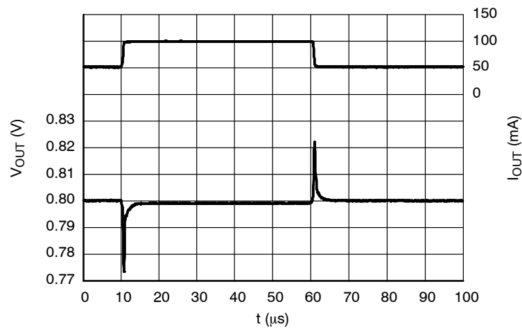
Figure 39. Load Transients, 0.8 V Version, I_{OUT} = 50 - 100 mA, t_R = t_F = 0.5 \mu s, V_{IN} = 1.8 V
