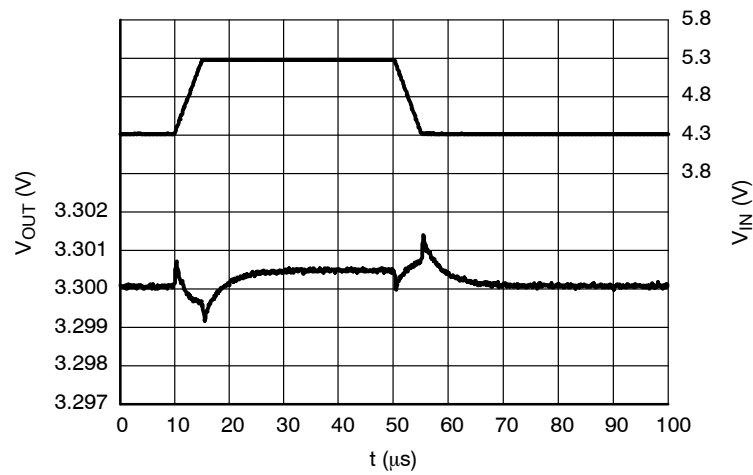
Figure 38. Line Transients, 3.3 V Version, t_R = t_F = 5 \mu s, I_{OUT} = 30 mA
