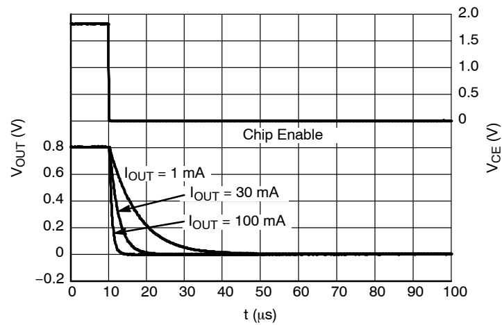
Figure 51. Shutdown, 0.8 V Version D, V_{IN} = 1.8\text{ V}
