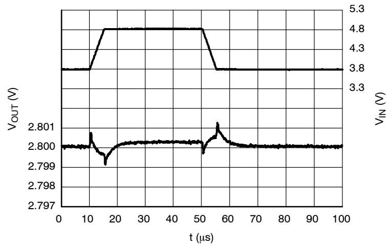
Figure 37. Line Transients, 2.8 V Version, t_R = t_F = 5 \mu s, I_{OUT} = 30 mA
