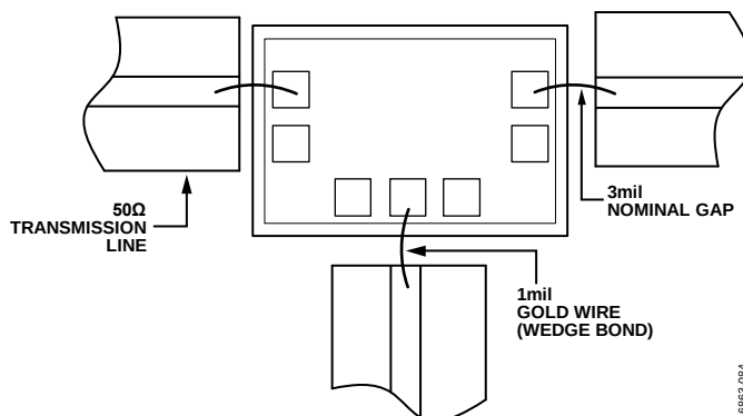
Figure 78. Assembly Diagram
