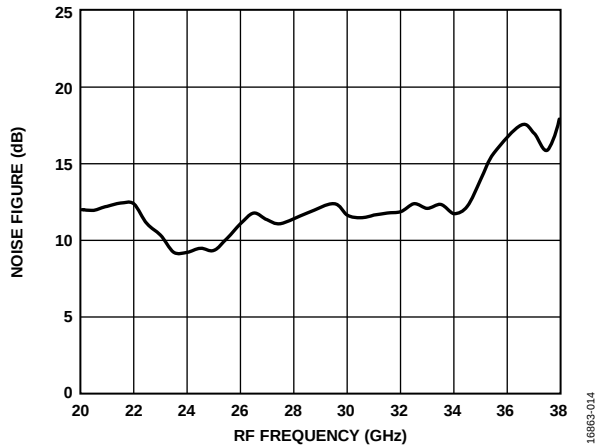
Figure 14. Noise Figure vs. RF Frequency at T_A = 25^\circ\text{C} , LO = 13 \text{ dBm}
