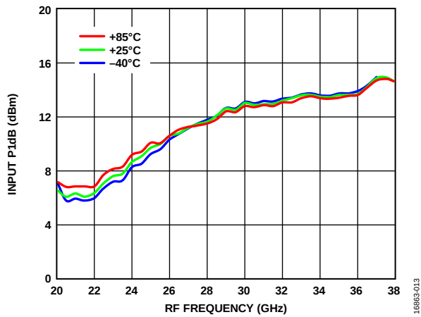
Figure 13. Input P1dB vs. RF Frequency at Various Temperatures, LO = 13 \text{ dBm}
