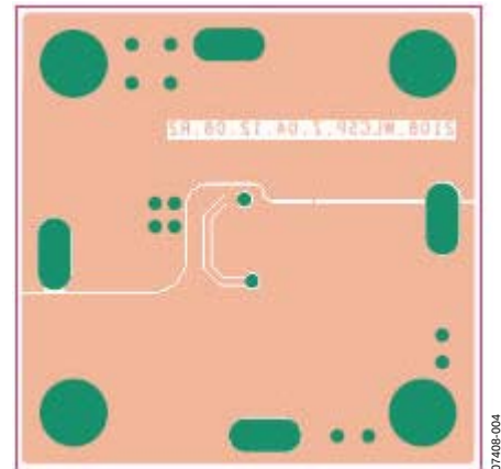
Figure 12. Bottom Layer, Recommended Layout for WLCSP
