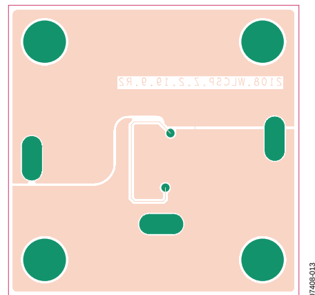
Figure 13. Bottom Layer, Recommended Layout for TSOT
