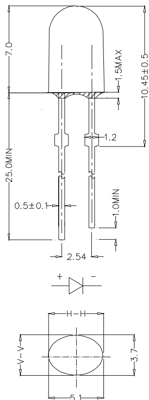
C5SMF-RJS/GJS/BJS&C5SME-RJS:
