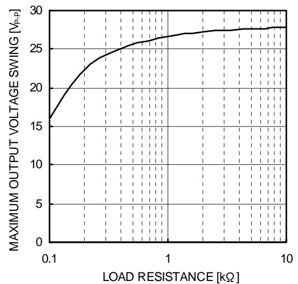
Figure 5. Maximum Output Voltage Swing - Load Resistance ( V_{CC}/V_{EE} = +15V/-15V, T_a = 25^\circ\text{C} )
