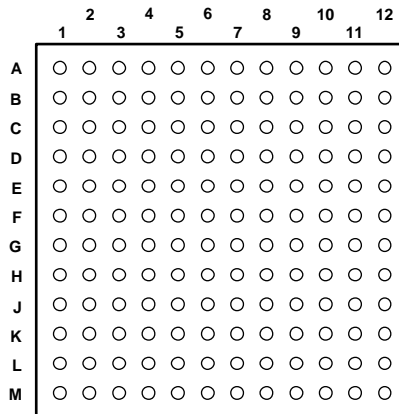
TOP VIEW (Not to Scale) Figure 5. BGA Pin Configuration
