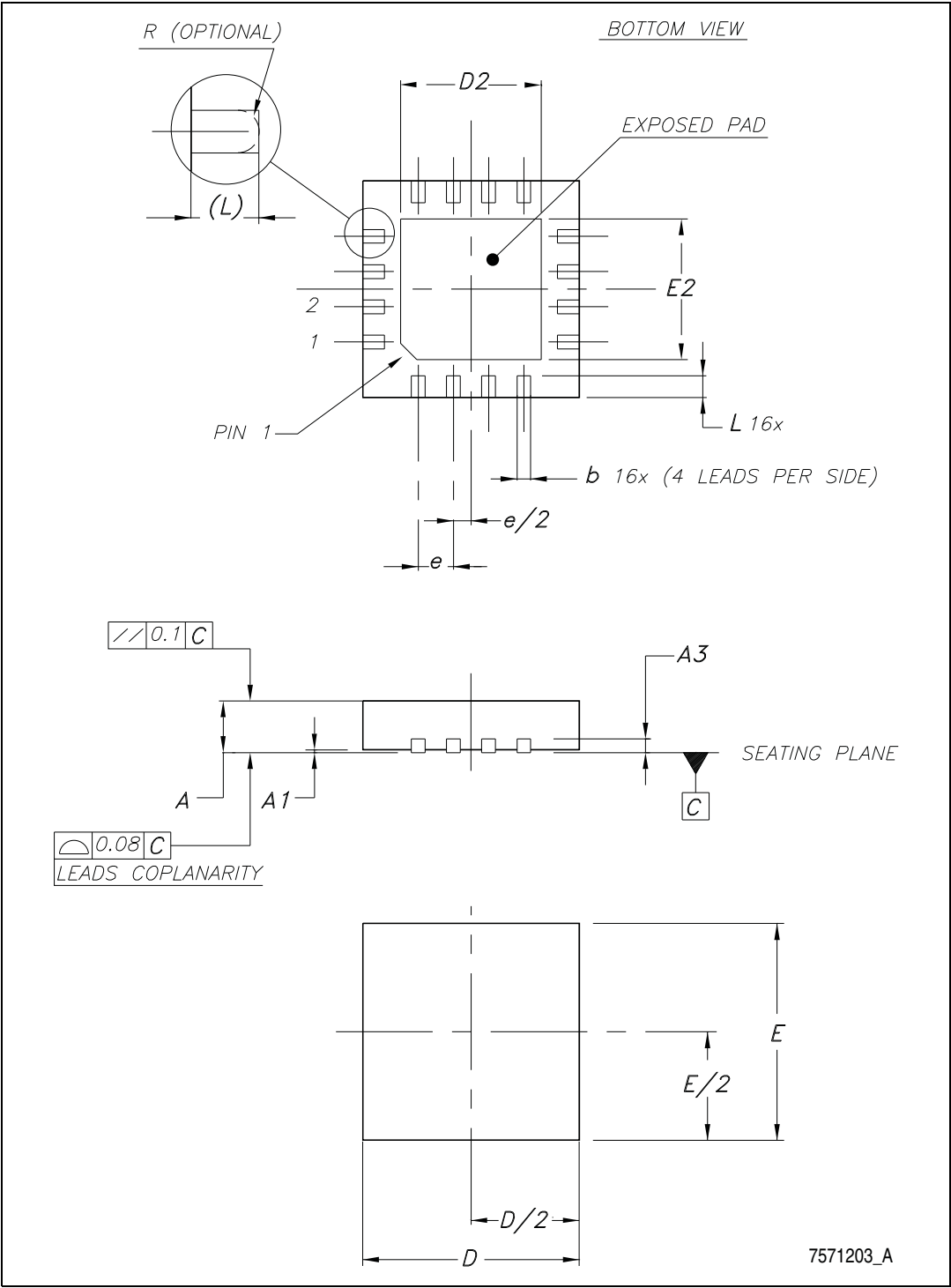
Figure 12. QFN16 (4 x 4 mm) drawing
