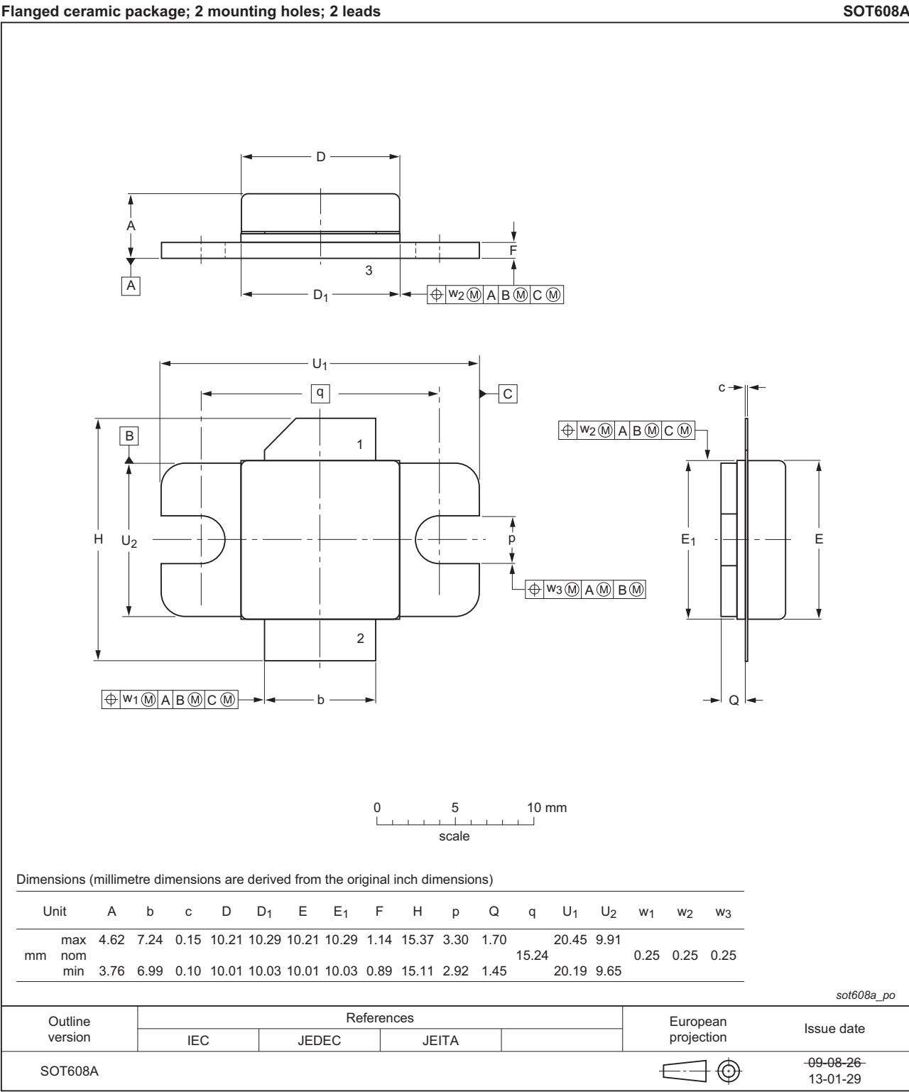
Fig 8. Package outline SOT608A
