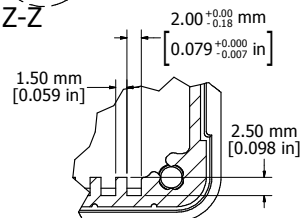
DETAIL AA
