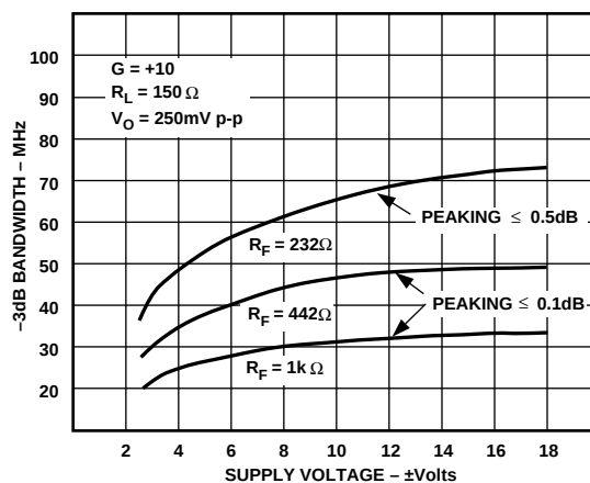
Figure 16. -3 \text{ dB} Bandwidth vs. Supply Voltage, Gain = +10, R_L = 150 \Omega
