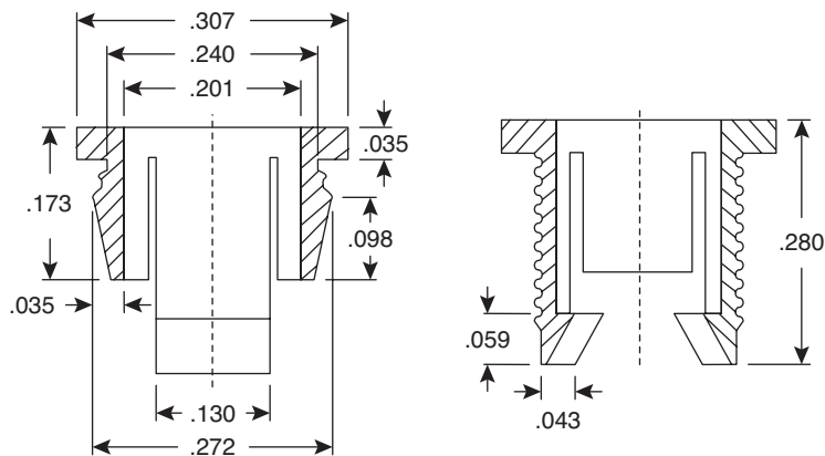
Dimensions (In.)
