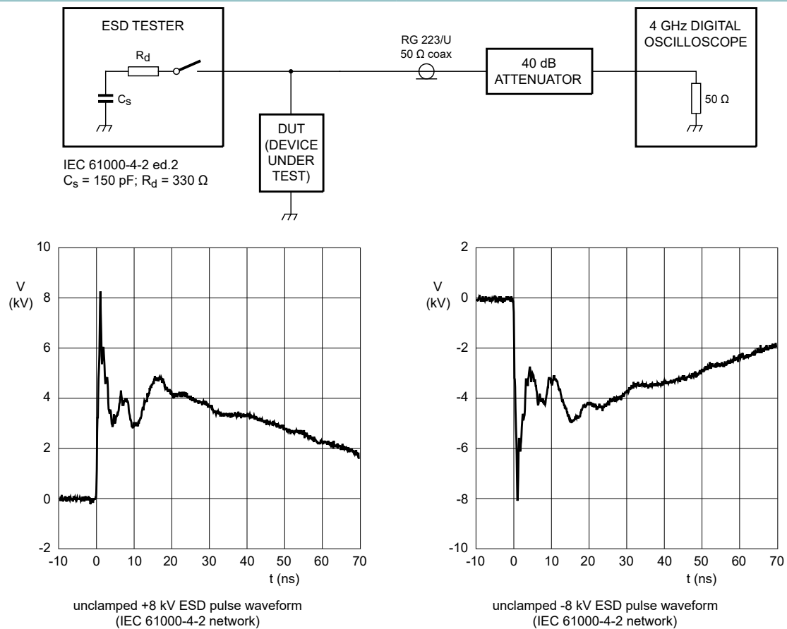
Fig. 12. ESD clamping test setup and waveforms
