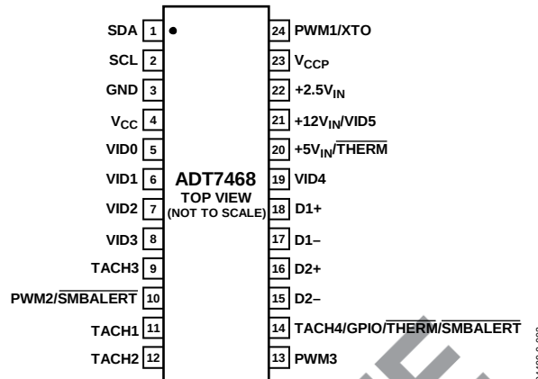
Figure 3. Pin Configuration
