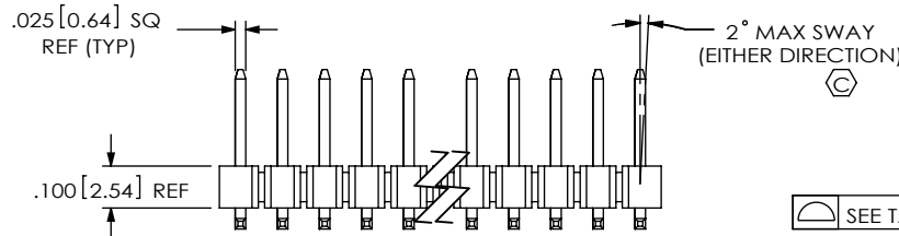
FIG 1 TSM-1XX-XX-XXX-DV SHOWN
