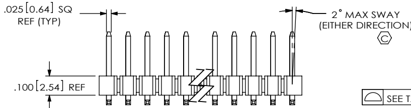
FIG 1 TSM-1XX-XX-XXX-DV SHOWN
