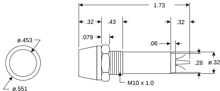
Dimensions (In.)
