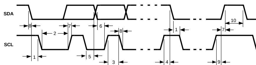
Figure 4-5. I²C Timing Diagram
