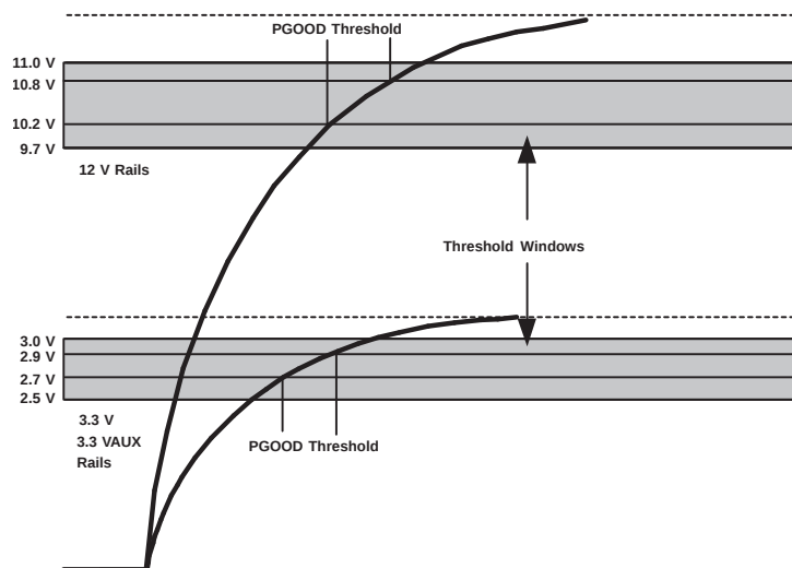
Figure 1. PGOOD Threshold, Grey Area is the PCIe Express CEM 1.1 Standard
