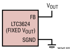
Figure 2. Setting the Output Voltage (Fixed V_{OUT} Option)
