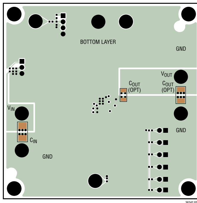
Figure 3b. Sample PCB Layout-Bottom Side
