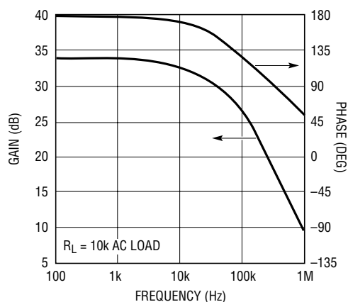
Error Amplifier Gain-Phase
