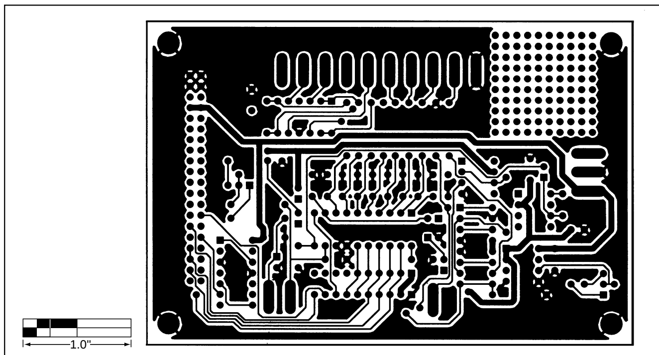
Figure 4. MAX147EV Kit PC Board Layout—Solder Side
