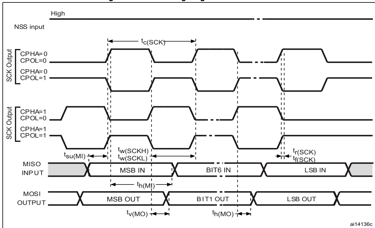
Figure 41. SPI1 timing diagram - master mode
