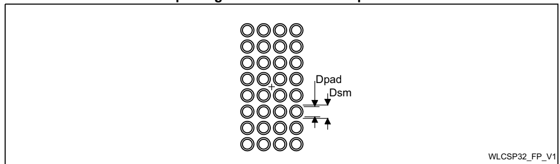
Figure 61. WLCSP32 - 32-ball, 1.913 x 3.329 mm, 0.4 mm pitch wafer level chip scale package recommended footprint
