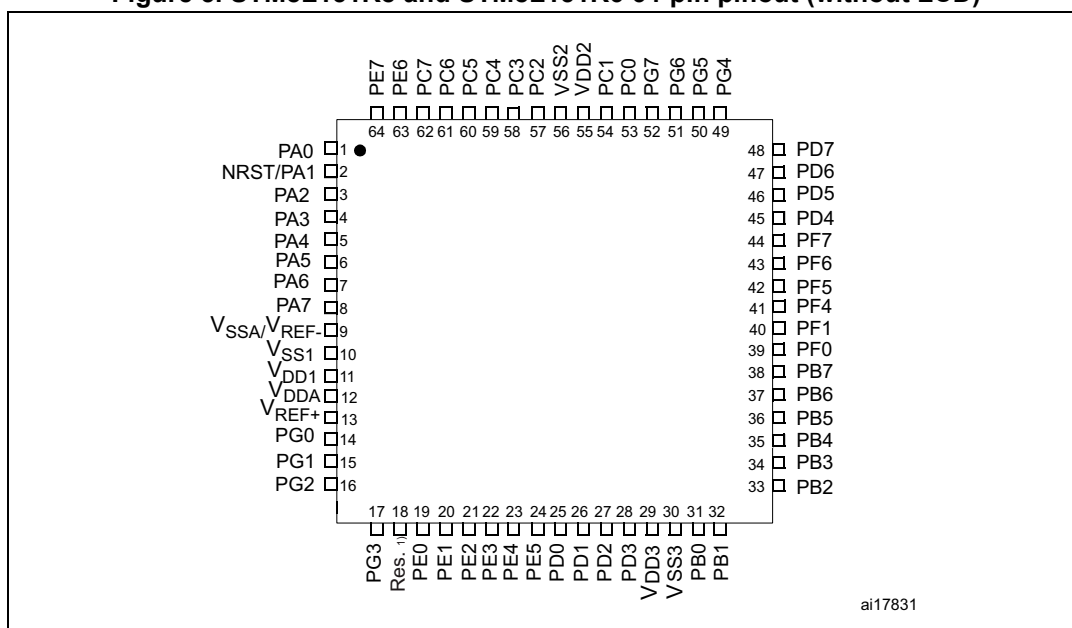
Figure 5. STM8L151R8 and STM8L151R6 64-pin pinout (without LCD)
