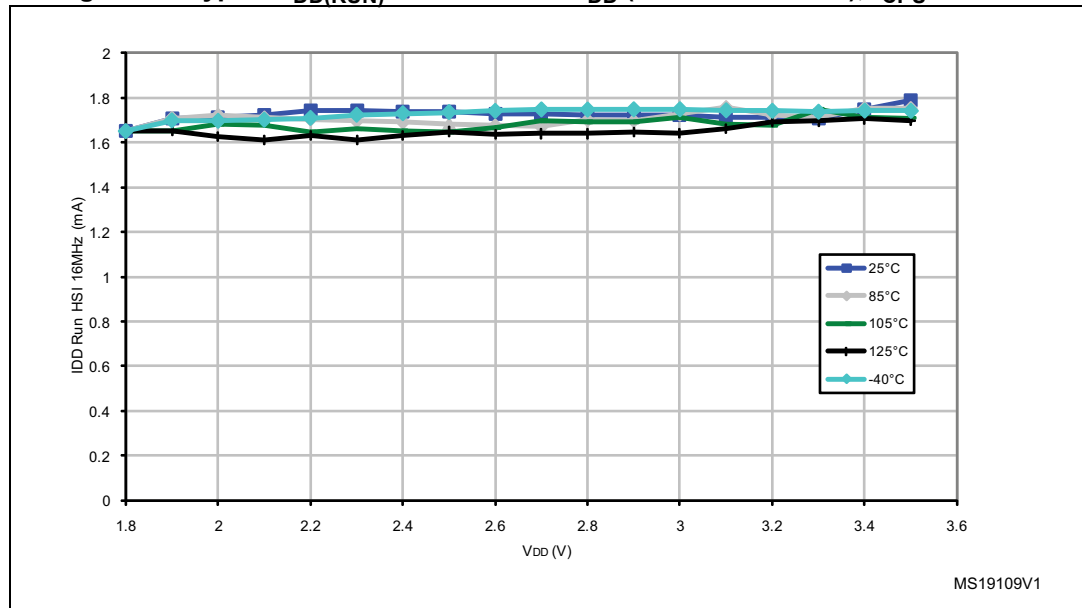
Figure 14. Typical I_{DD(RUN)} from RAM vs. V_{DD} (HSI clock source), f_{CPU} = 16 MHz
