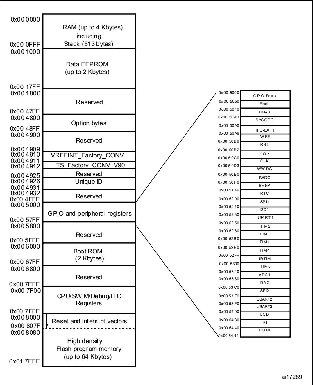
Figure 10. Memory map
