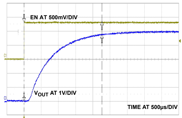
FIGURE 8. START-UP WAVEFORM
