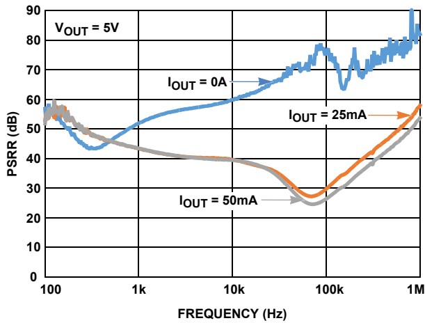
FIGURE 11. PSRR vs FREQUENCY FOR VARIOUS LOAD CURRENT, V_{OUT} = 5V
