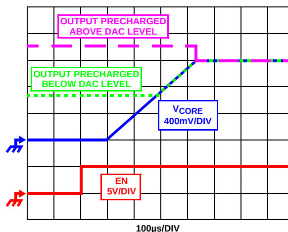
FIGURE 12. SOFT-START WAVEFORMS FOR ISL6324A-BASED MULTI-PHASE CONVERTER
