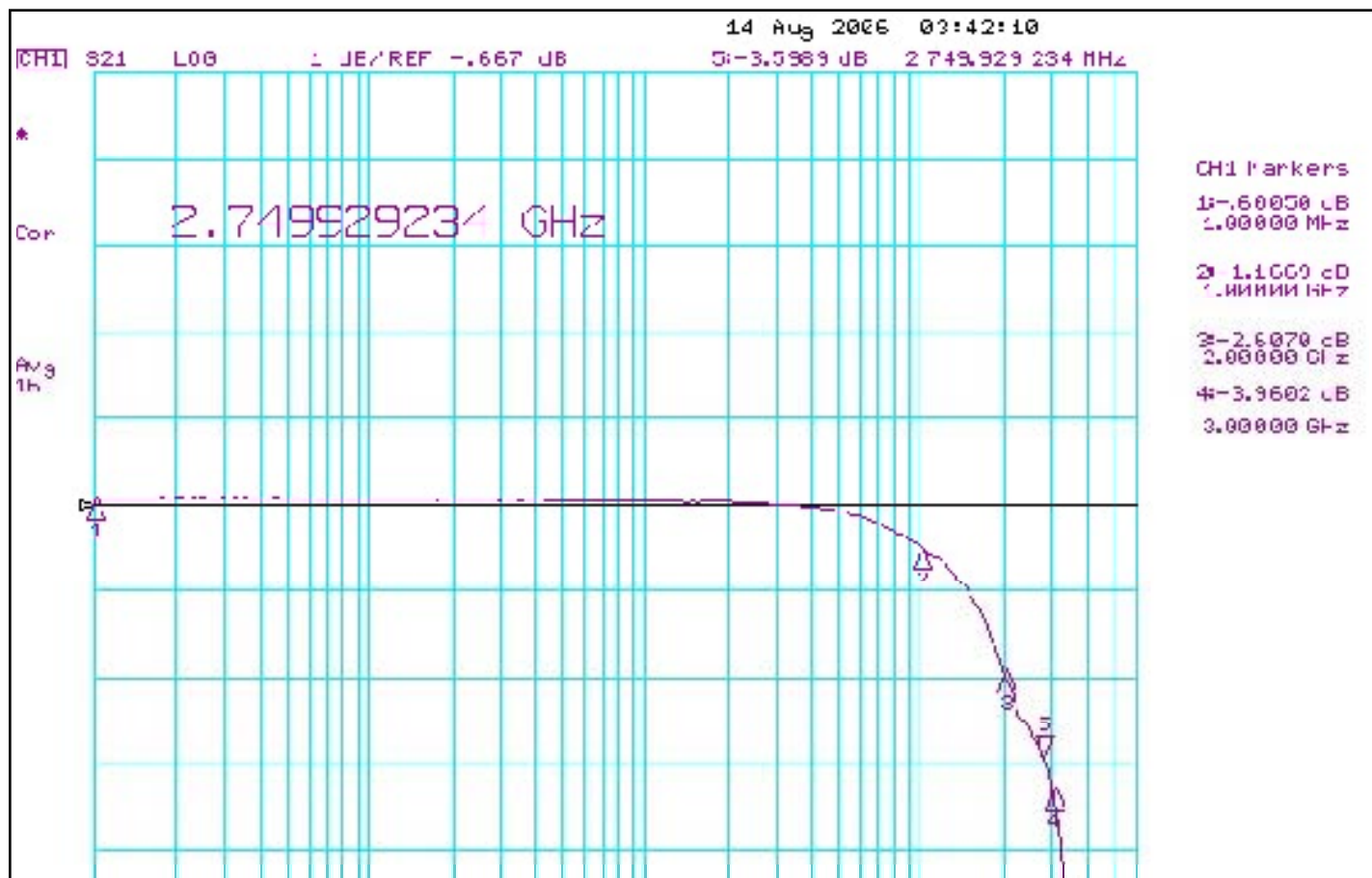
Fig 5. Insertion Loss
