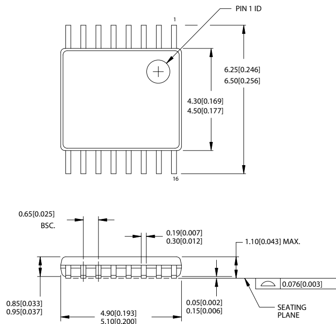
Figure 10. 16-Pin TSSOP 4.40 mm Body Z16 and ZZ16
