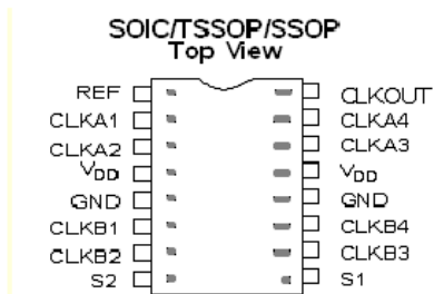
Figure 1. Pin Configuration – CY23S09
