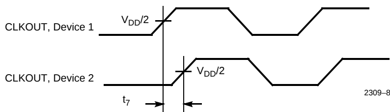
Figure 7. Device-Device Skew
