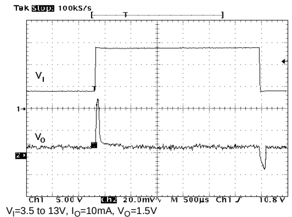
Figure 18: Line Transient
