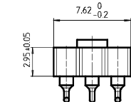
Dimensions of Pick-and-Place pad for 3 pole strip
