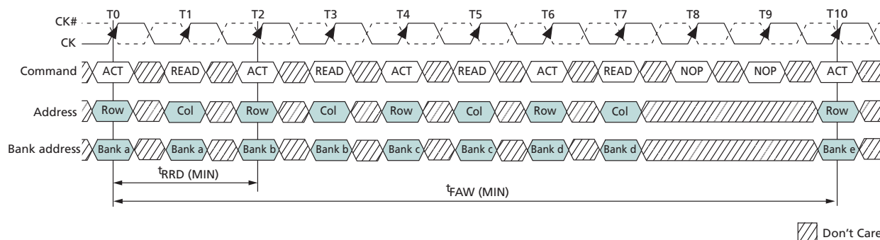
Figure 43: Multibank Activate Restriction
