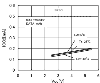
Fig.11 Current consumption at READ action ICC2 ( f_{SCL}=400\text{kHz} )
