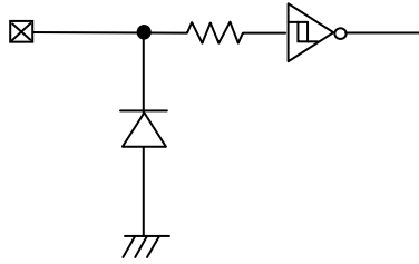
Fig.54 Input pin circuit diagram
