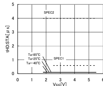
Fig.19 Start condition hold time t_{HD:STA}
