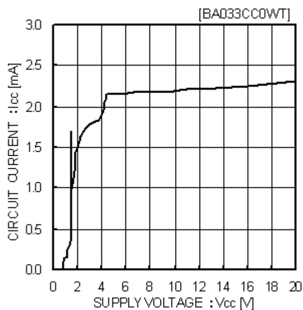
Fig.3 Circuit current
