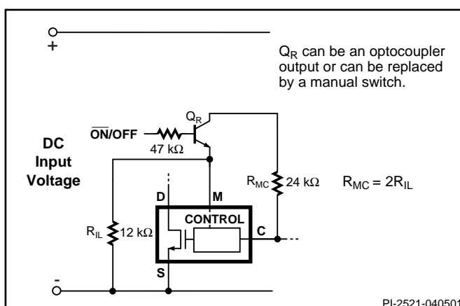
Figure 39. Active-off Remote ON/OFF with Externally Set Current Limit.
