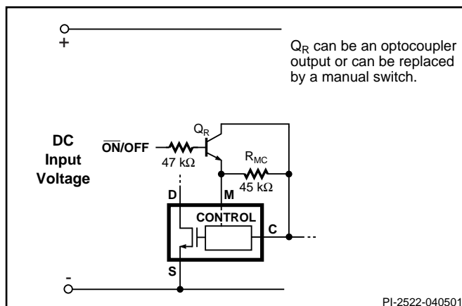
Figure 37. Active-off Remote ON/OFF. Maximum Duty Cycle will be Reduced.
