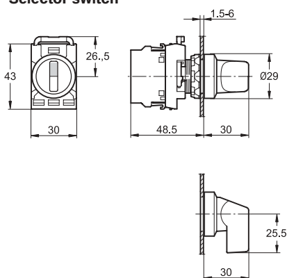
Selector switch
