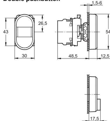
Double pushbutton
