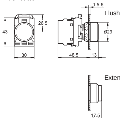
Pushbutton
