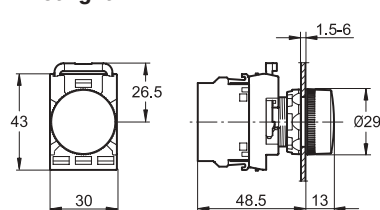
Pilot light
