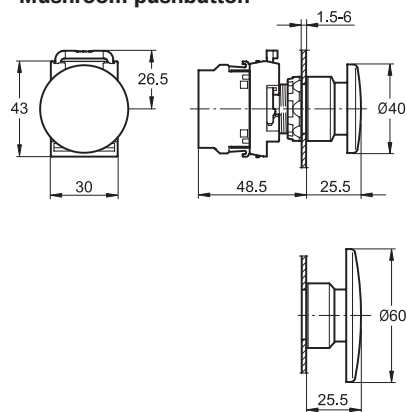
Mushroom pushbutton
