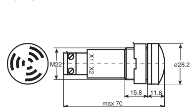
Buzzer
