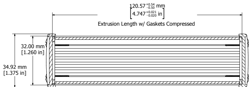
SECTION Y-Y
