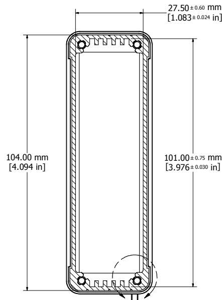
SECTION T-T
