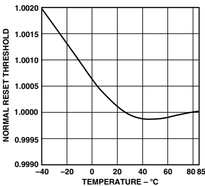
TPC 5. Normalized Reset Voltage Threshold vs. Temperature
