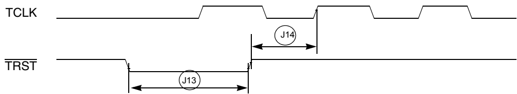
Figure 32. \overline{TRST} Timing
