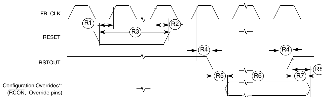
Figure 22. \overline{\text{RESET}} and Configuration Override Timing
