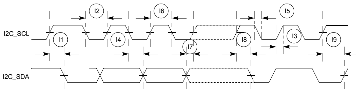
Figure 23. I²C Input/Output Timings
