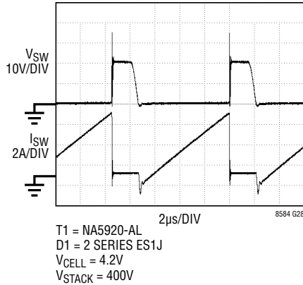
Switching Waveform
