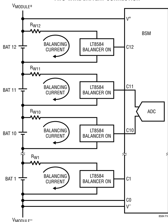
Figure 16. LT8584 Battery Connections
