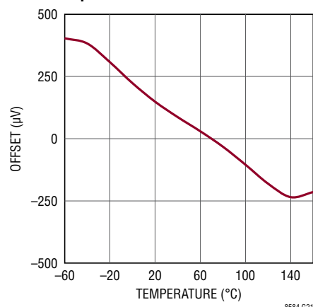
V_{SNS} Amplifier Input Referred Offset
