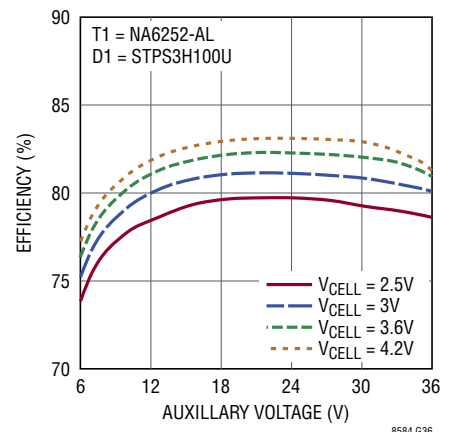
Conversion Efficiency
