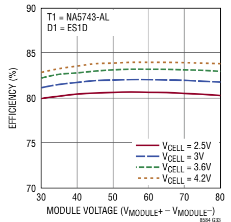
Conversion Efficiency
