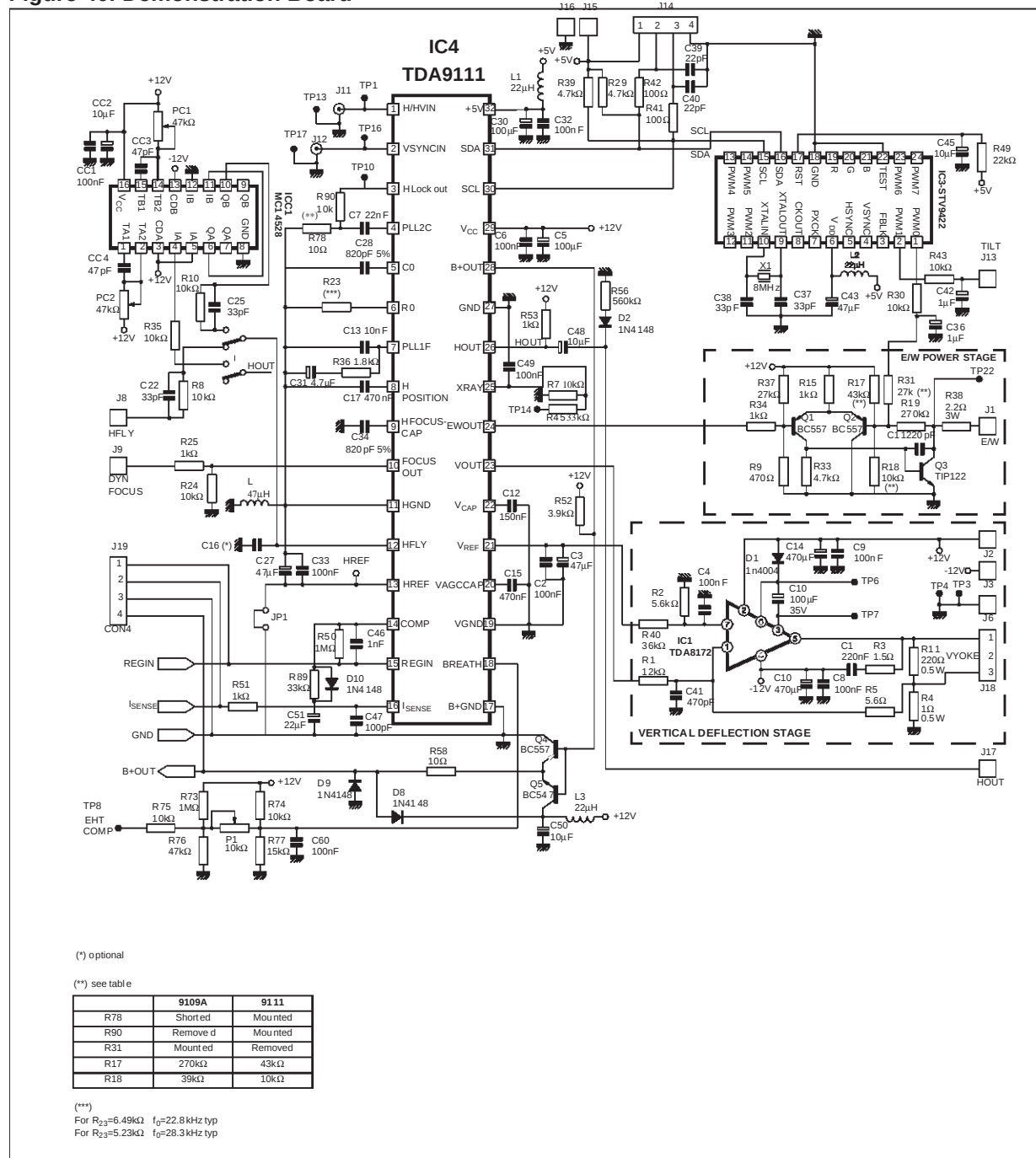
Figure 40. Demonstration Board
