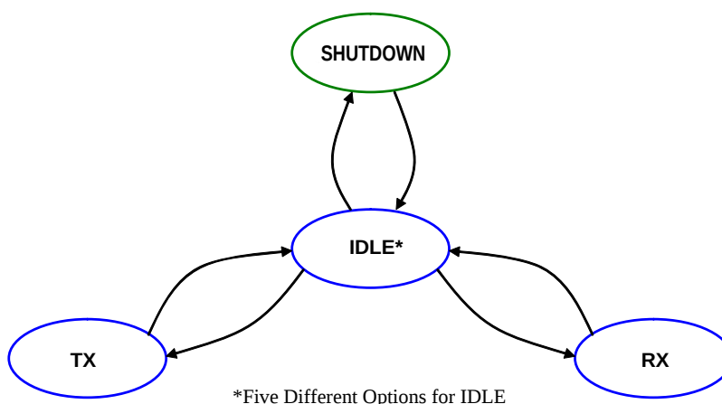
Figure 23.1. State Machine Diagram
