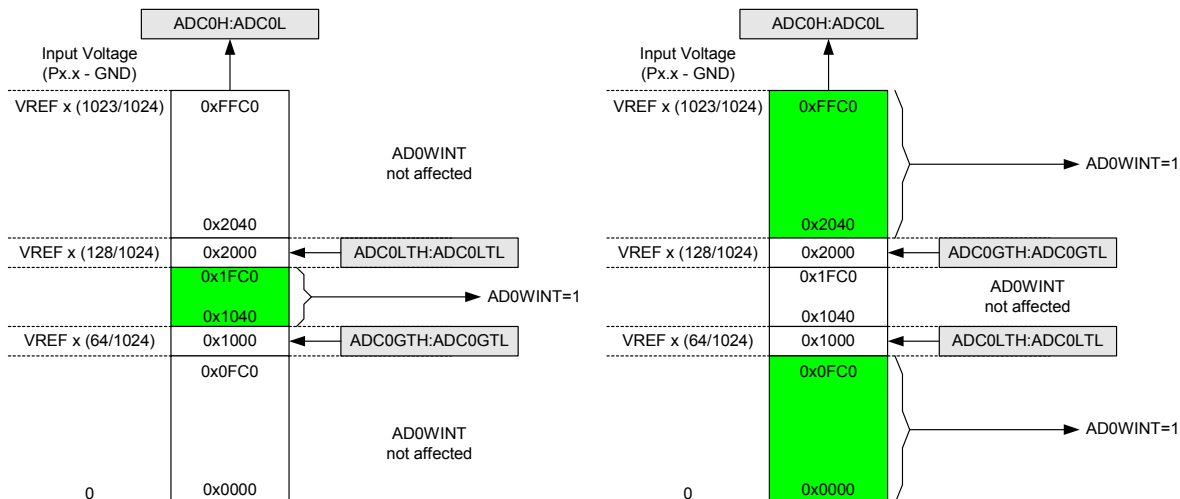
Figure 5.6. ADC Window Compare Example: Left-Justified Single-Ended Data
