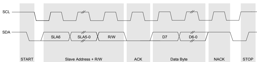
Figure 24.3. SMBus Transaction
