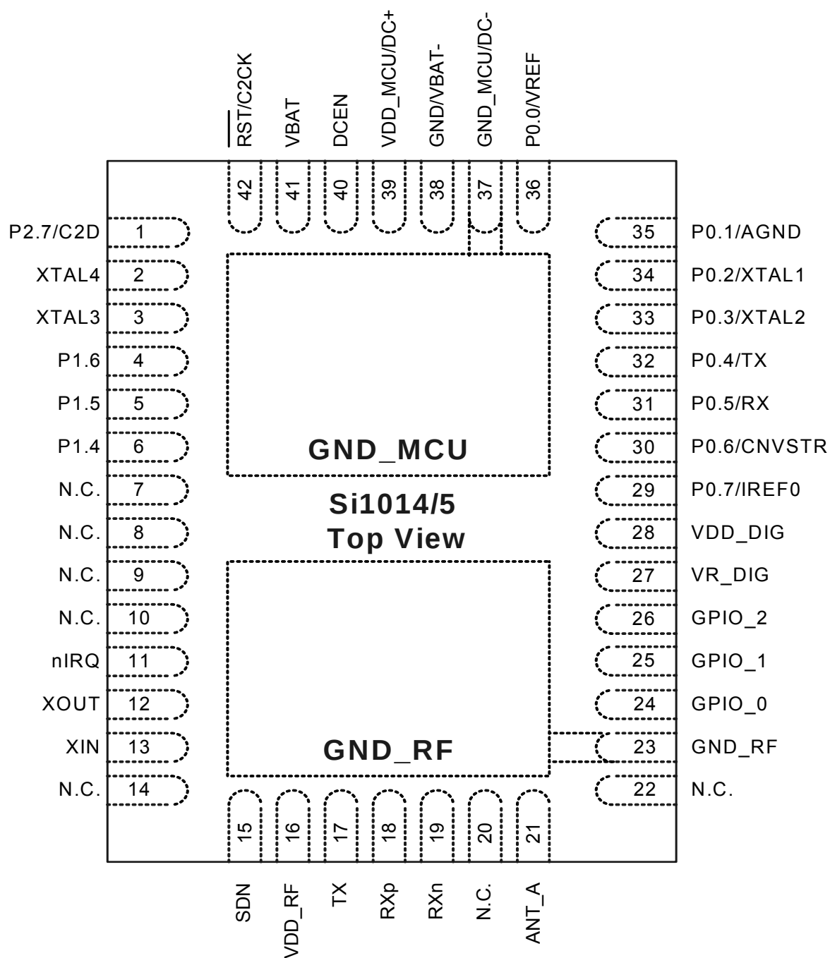
Figure 3.2. Si1004/5 Pinout Diagram (Top View)
