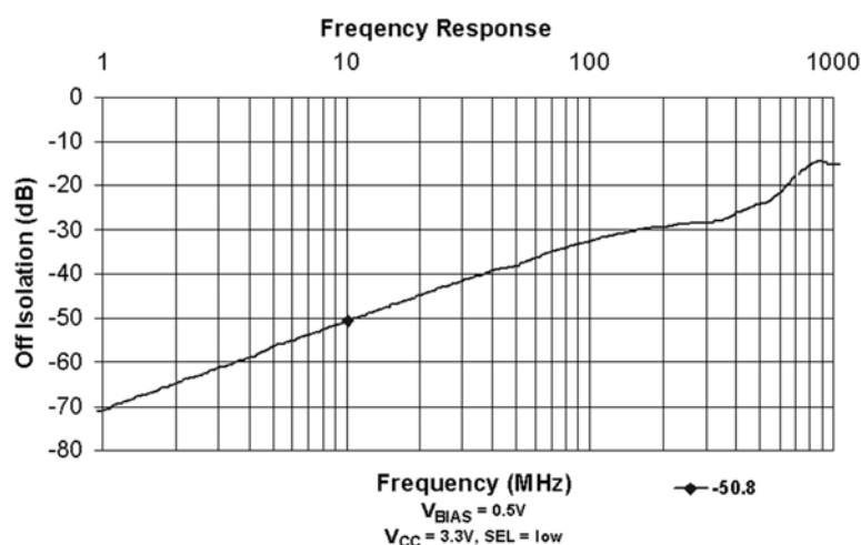
FIGURE 4. OFF Isolation
