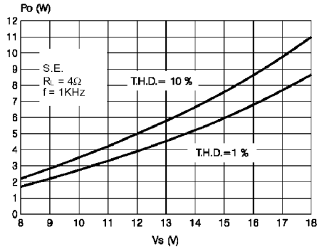
Figure 12. Output Power vs. Supply Voltage
