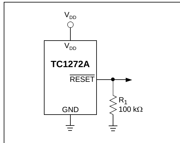
FIGURE 3-2: The addition of R_1 at the \overline{\text{RESET}} output of the TC1272A ensures that the \overline{\text{RESET}} output is valid to V_{DD} = 0V .
