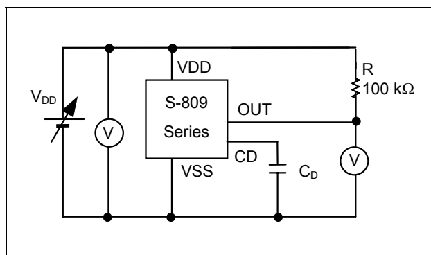
Figure 25 Measurement Circuit for Delay Time
