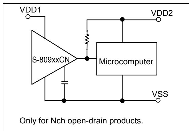
Figure 27 Example for Reset Circuits(S-809xxCN)
