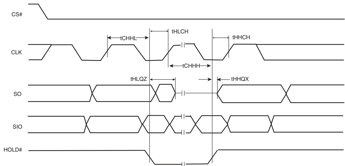
Figure 8.5 Hold Timing
