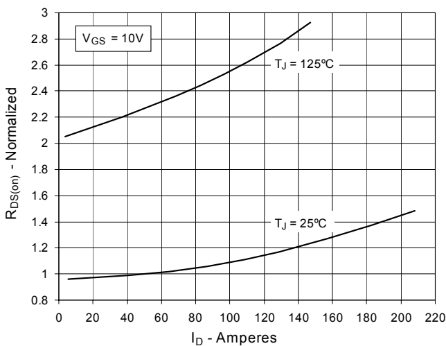
Fig. 5. R_{DS(on)} Normalized to I_D = 50\text{A} Value vs. Drain Current
