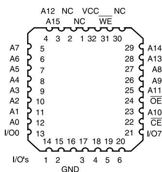
PLCC Top View
